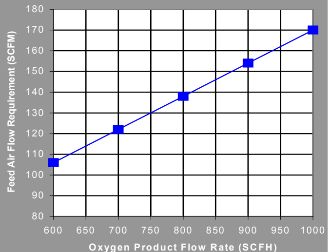
AirSep "AS-K" Oxygen Generator Feed Air Requirement (93% nominal oxygen)
