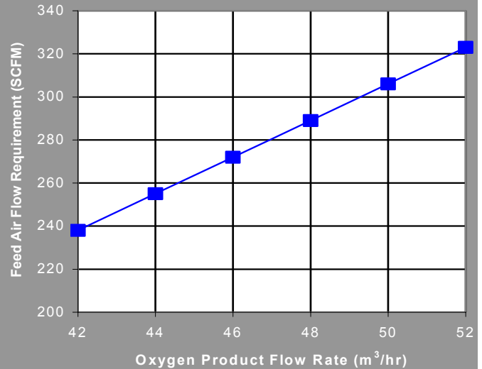
AirSep "AS-N" Oxygen Generator Feed Air Requirement (93% nominal oxygen)
